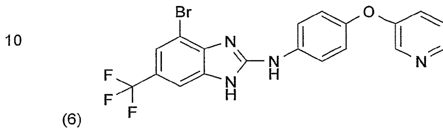
(4-Brom-6-trifluormethyl-1H-benzimidazol-2-yl)-[4-(pyridin-3-yloxy)-phenyl]-amin
